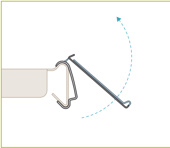
The 127 Series | Hinged molding swings up for ease of access
